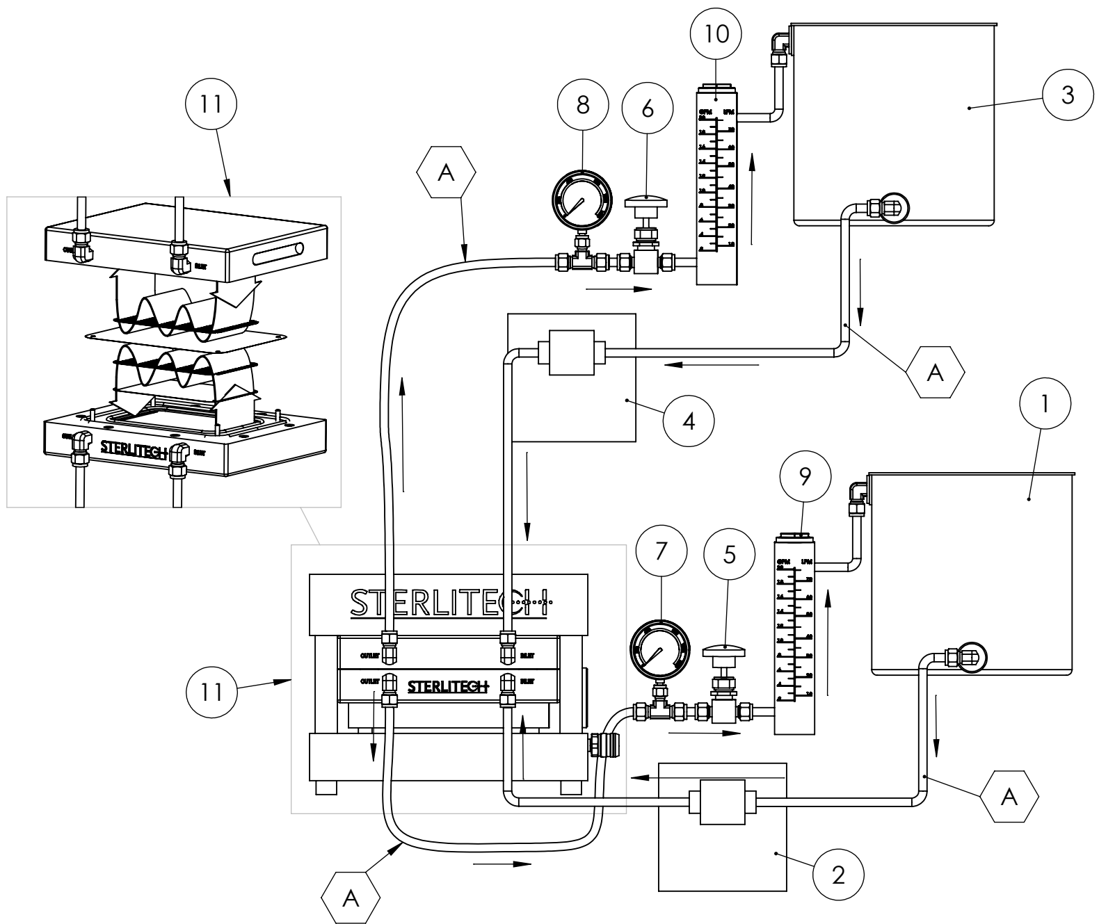
Sopa FO Flow Diagram
